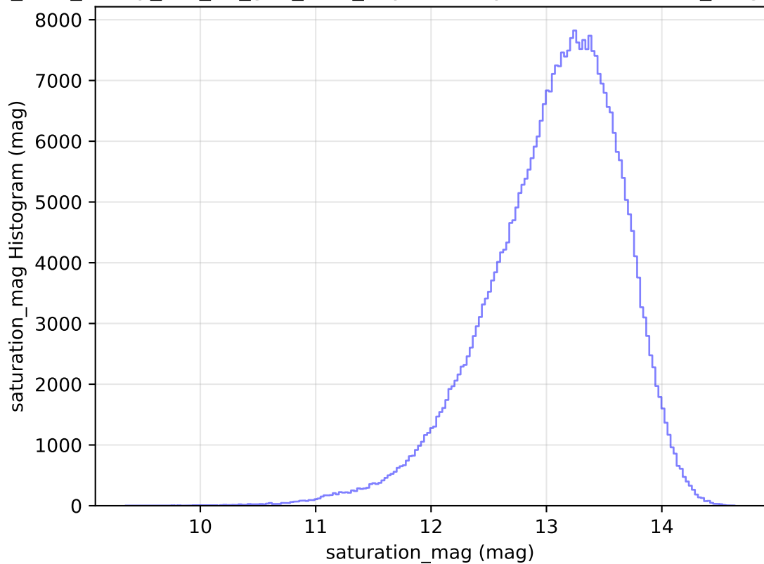
too_elab_heavy_r64_d3_griz_v3.4_10yrs WFD y band: saturation_mag Histogram
