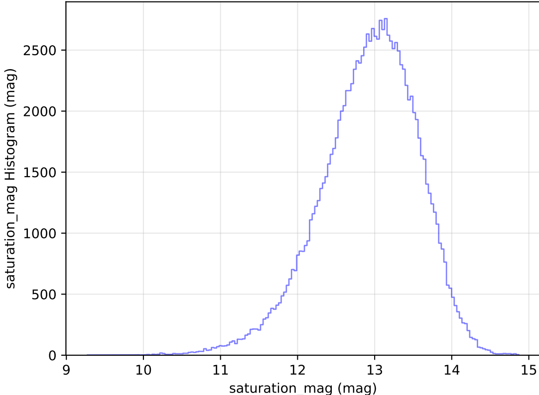
too_elab_heavy_r64_d3_griz_v3.4_10yrs WFD u band: saturation_mag Histogram
