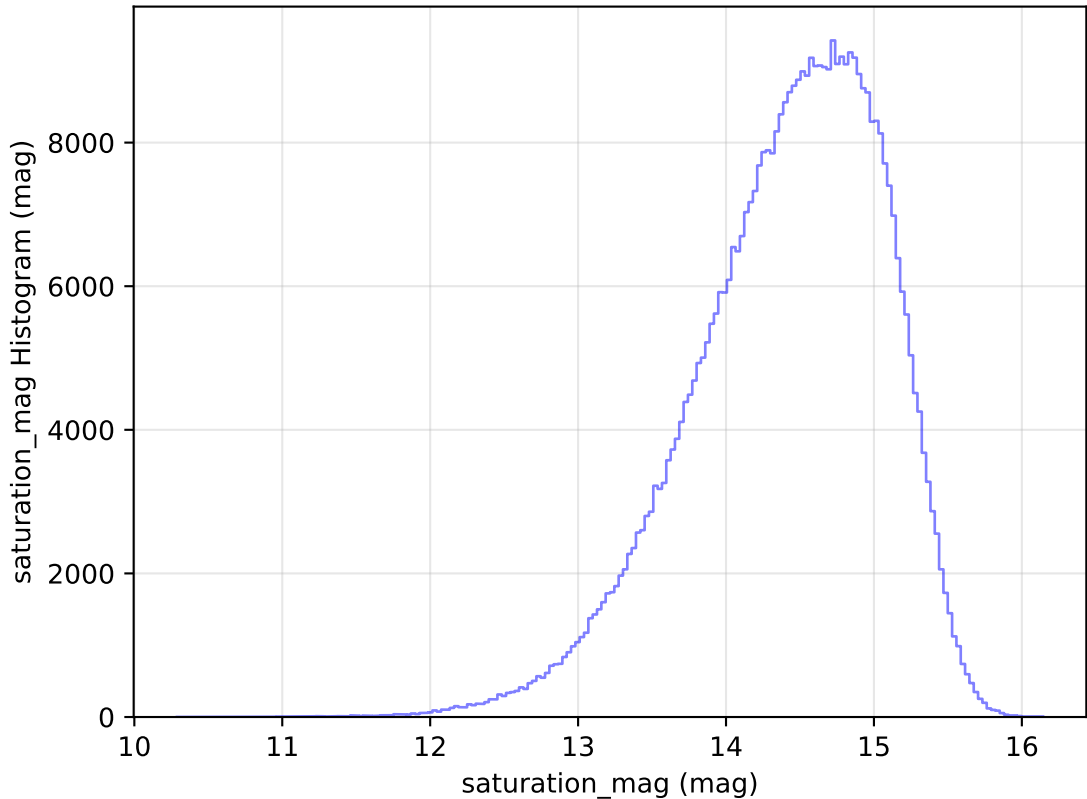
too_elab_heavy_r64_d3_griz_v3.4_10yrs WFD i band: saturation_mag Histogram
