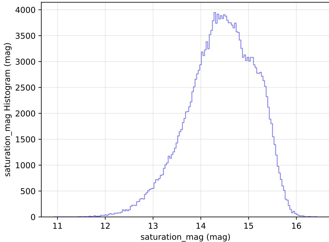
too_elab_heavy_r64_d3_griz_v3.4_10yrs WFD g band: saturation_mag Histogram
