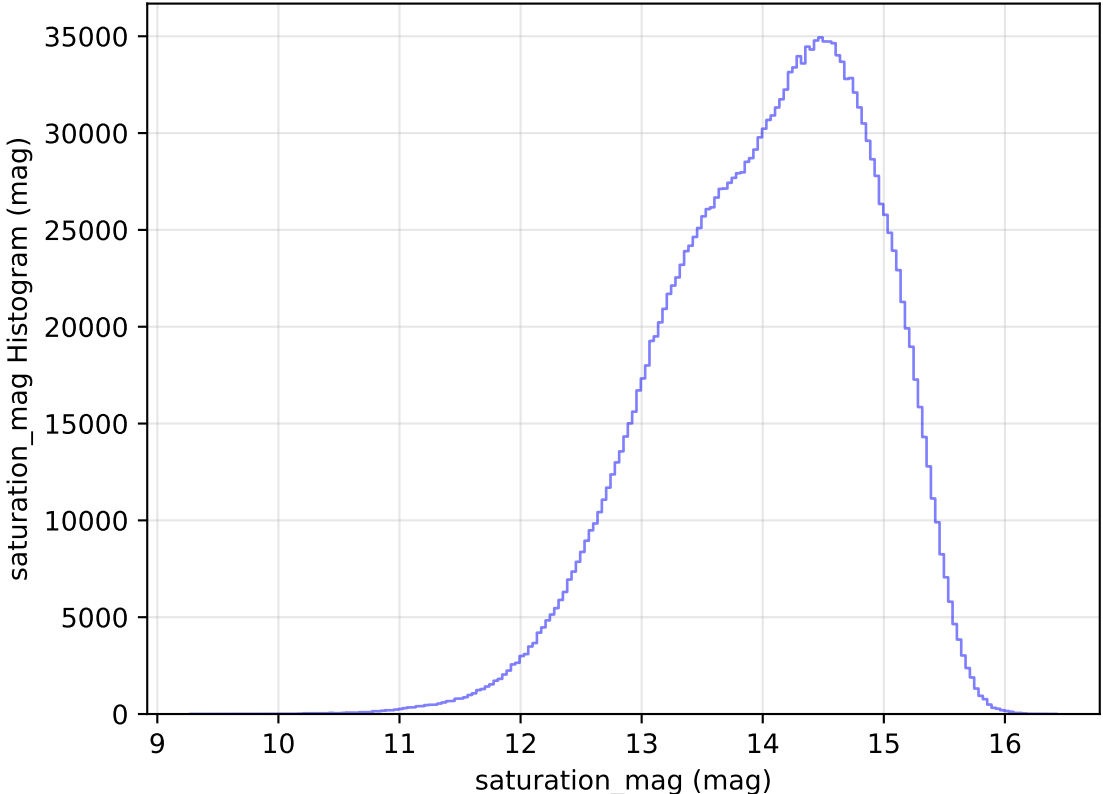
too_elab_heavy_r64_d3_griz_v3.4_10yrs WFD all bands: saturation_mag Histogram
