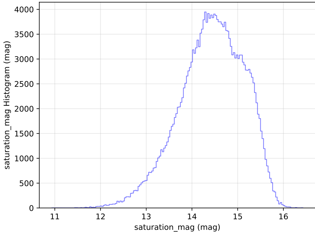
too_elab_heavy_r64_d3_griz_v3.4_10yrs All sky g band: saturation_mag Histogram
