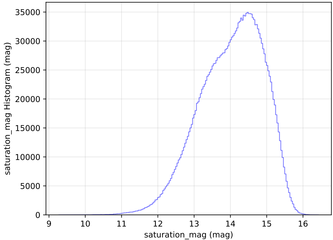
too_elab_heavy_r64_d3_griz_v3.4_10yrs All sky all bands: saturation_mag Histogram
