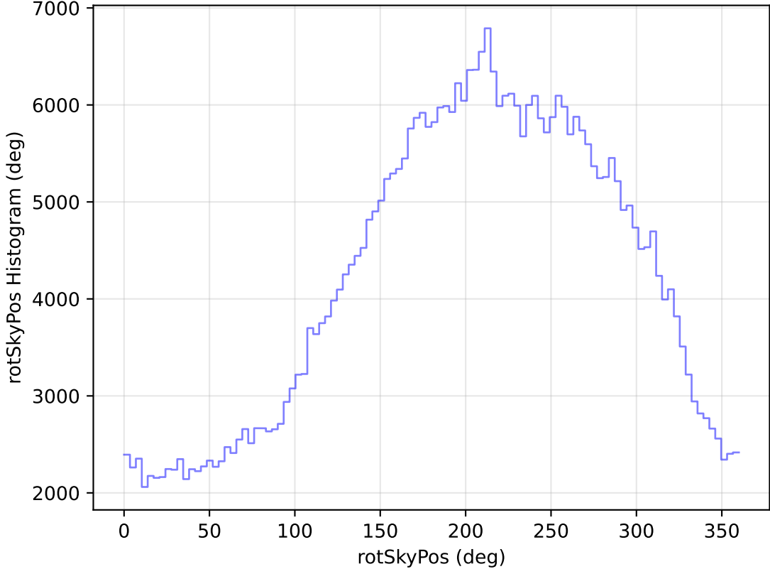
too_elab_heavy_r64_d3_griz_v3.4_10yrs WFD z band: rotSkyPos Histogram
