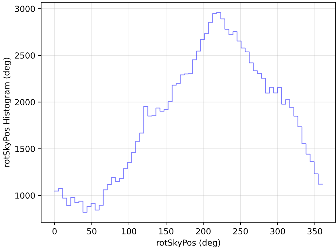
too_elab_heavy_r64_d3_griz_v3.4_10yrs WFD u band: rotSkyPos Histogram
