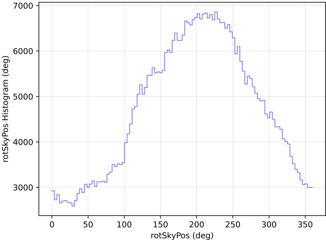
too_elab_heavy_r64_d3_griz_v3.4_10yrs WFD r band: rotSkyPos Histogram
