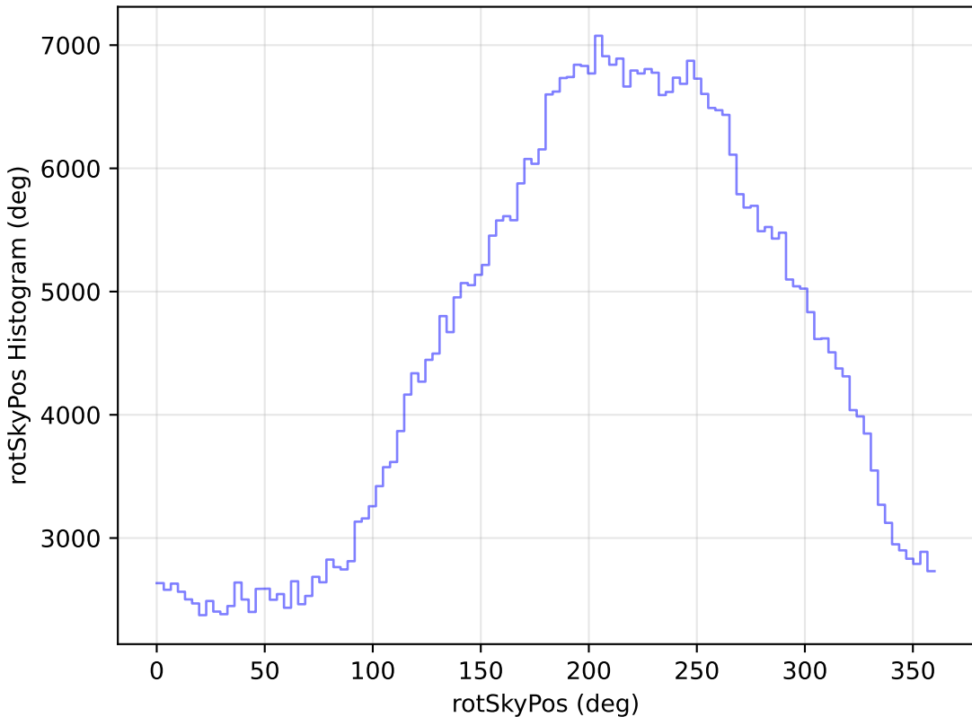
too_elab_heavy_r64_d3_griz_v3.4_10yrs WFD i band: rotSkyPos Histogram
