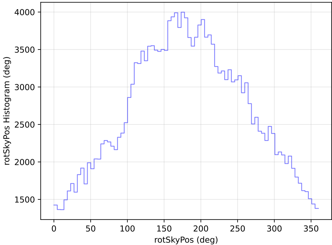
too_elab_heavy_r64_d3_griz_v3.4_10yrs WFD g band: rotSkyPos Histogram
