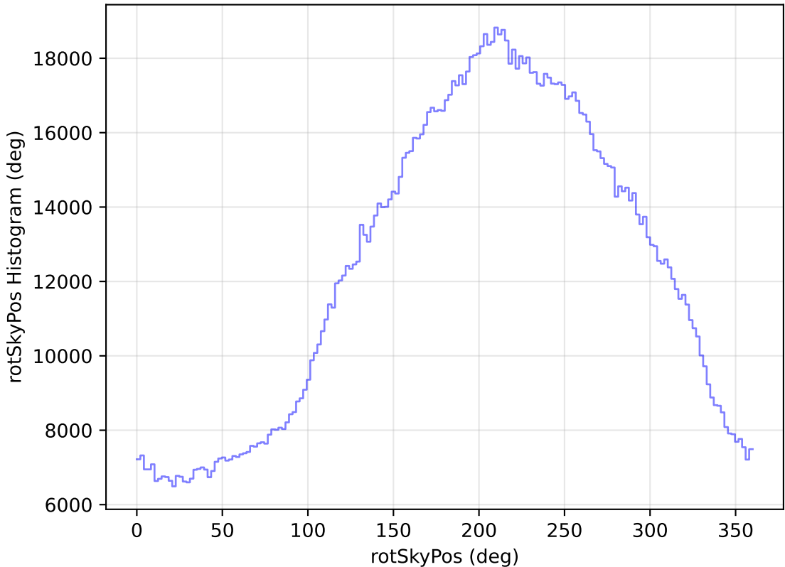
too_elab_heavy_r64_d3_griz_v3.4_10yrs WFD all bands: rotSkyPos Histogram
