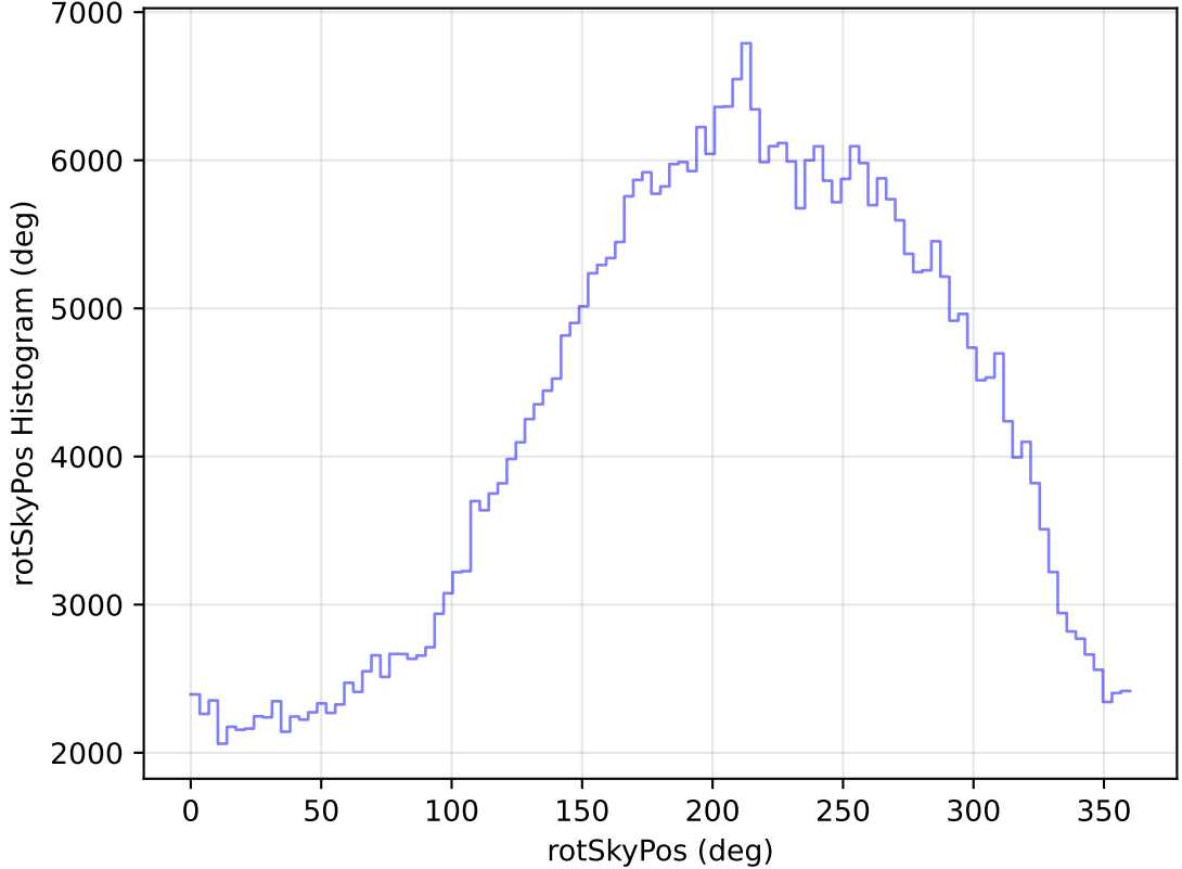
too_elab_heavy_r64_d3_griz_v3.4_10yrs All sky z band: rotSkyPos Histogram
