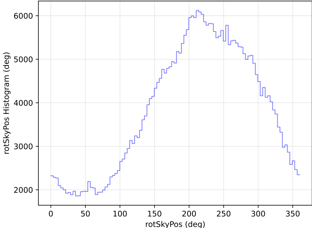
too_elab_heavy_r64_d3_griz_v3.4_10yrs All sky y band: rotSkyPos Histogram
