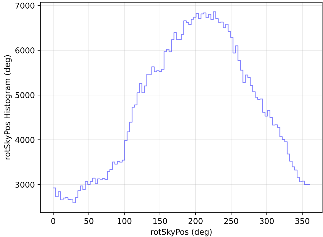
too_elab_heavy_r64_d3_griz_v3.4_10yrs All sky r band: rotSkyPos Histogram
