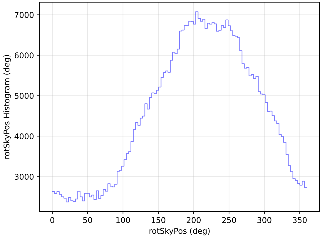
too_elab_heavy_r64_d3_griz_v3.4_10yrs All sky i band: rotSkyPos Histogram
