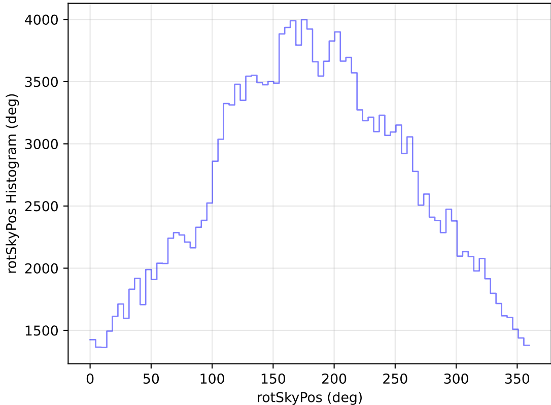
too_elab_heavy_r64_d3_griz_v3.4_10yrs All sky g band: rotSkyPos Histogram
