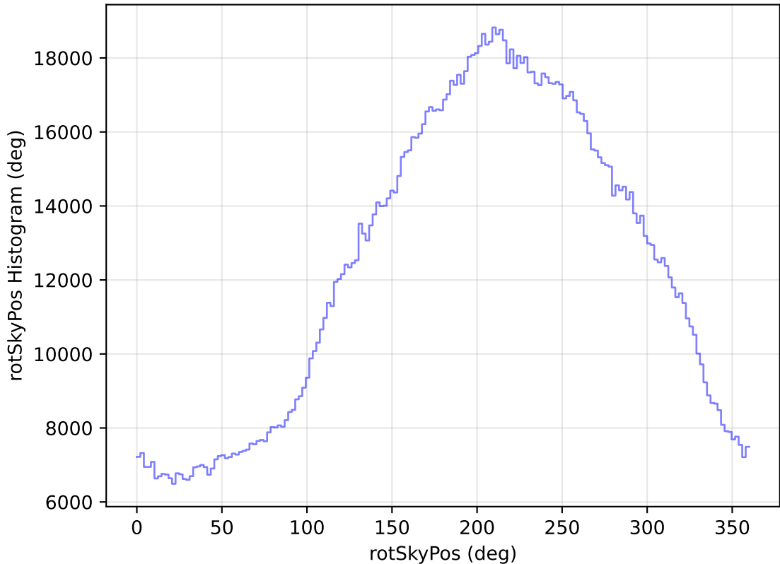
too_elab_heavy_r64_d3_griz_v3.4_10yrs All sky all bands: rotSkyPos Histogram
