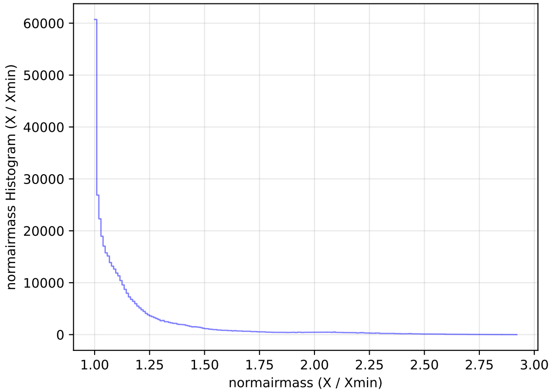
too_elab_heavy_r64_d3_griz_v3.4_10yrs WFD z band: normairmass Histogram
