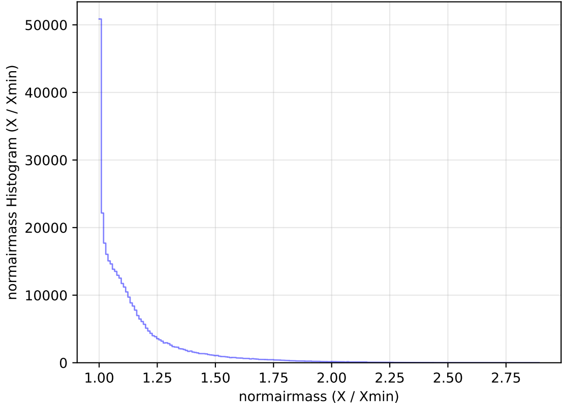
too_elab_heavy_r64_d3_griz_v3.4_10yrs WFD y band: normairmass Histogram
