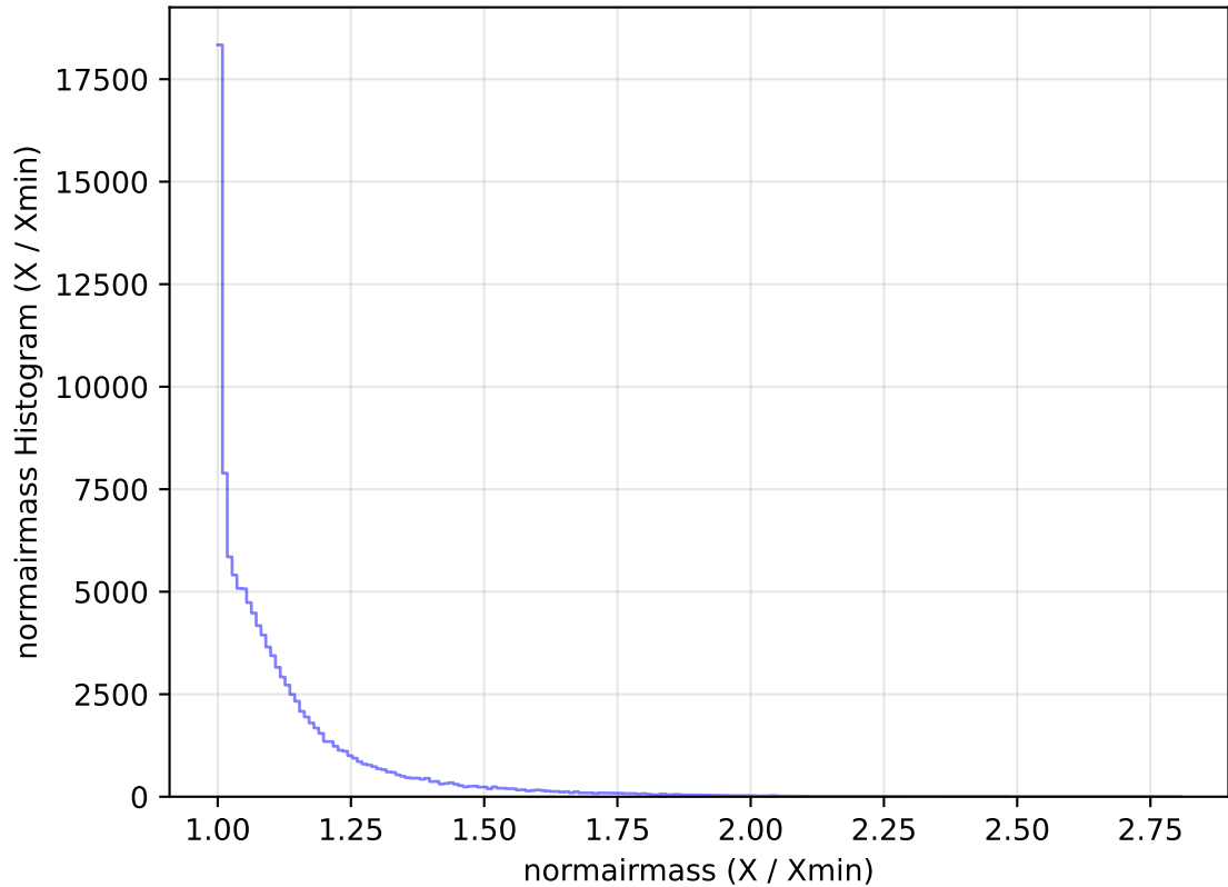
too_elab_heavy_r64_d3_griz_v3.4_10yrs WFD u band: normairmass Histogram
