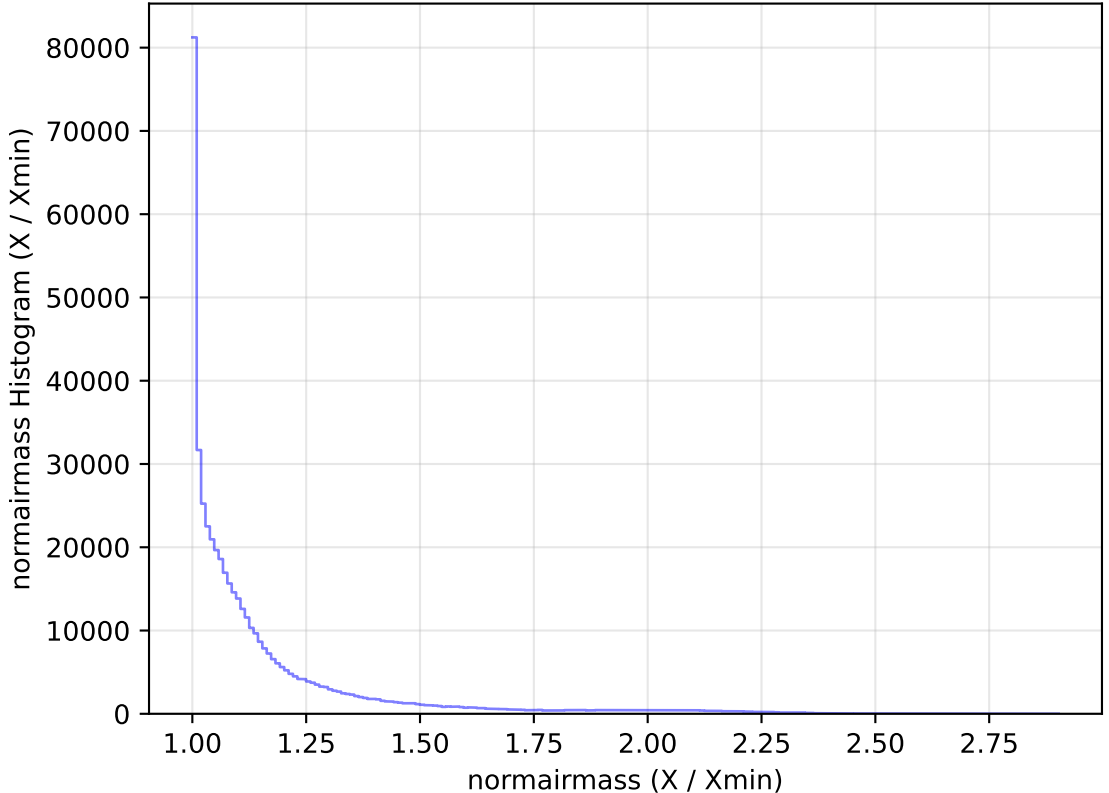
too_elab_heavy_r64_d3_griz_v3.4_10yrs WFD r band: normairmass Histogram
