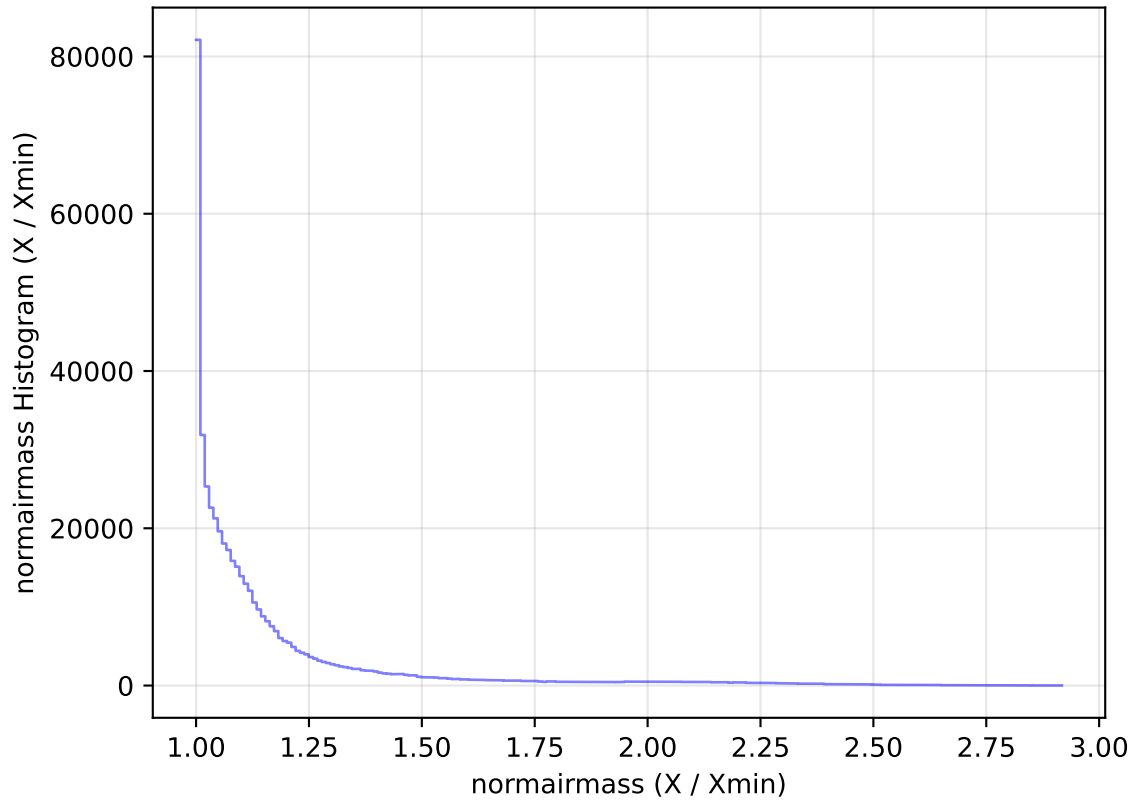
too_elab_heavy_r64_d3_griz_v3.4_10yrs WFD i band: normairmass Histogram
