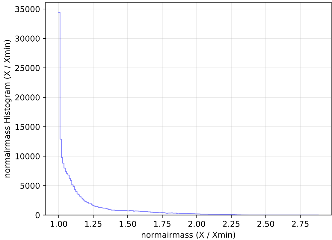
too_elab_heavy_r64_d3_griz_v3.4_10yrs WFD g band: normairmass Histogram
