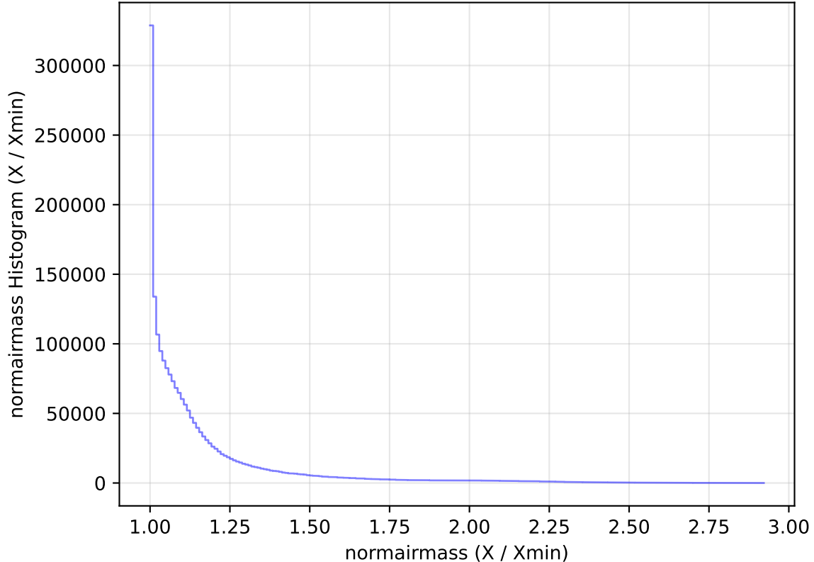
too_elab_heavy_r64_d3_griz_v3.4_10yrs WFD all bands: normairmass Histogram
