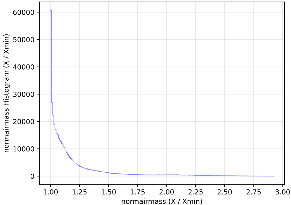
too_elab_heavy_r64_d3_griz_v3.4_10yrs All sky z band: normairmass Histogram
