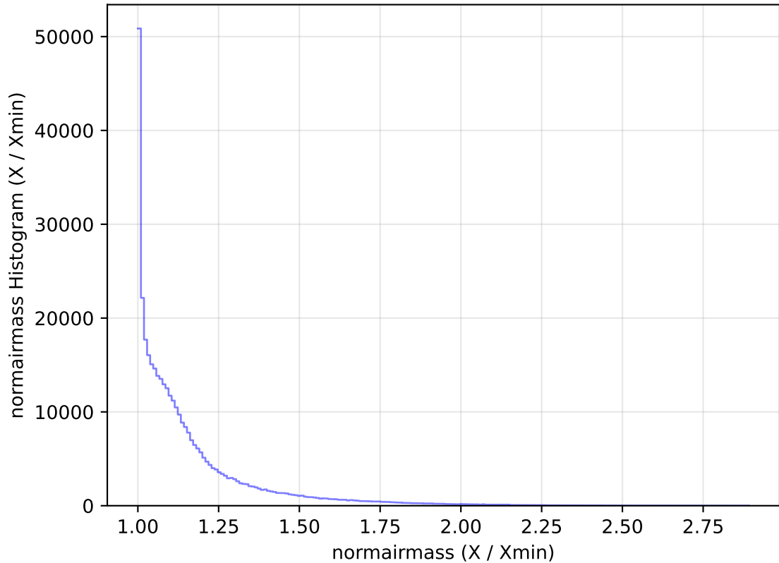
too_elab_heavy_r64_d3_griz_v3.4_10yrs All sky y band: normairmass Histogram
