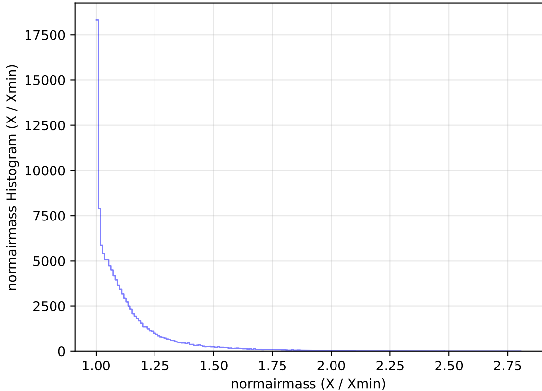
too_elab_heavy_r64_d3_griz_v3.4_10yrs All sky u band: normairmass Histogram
