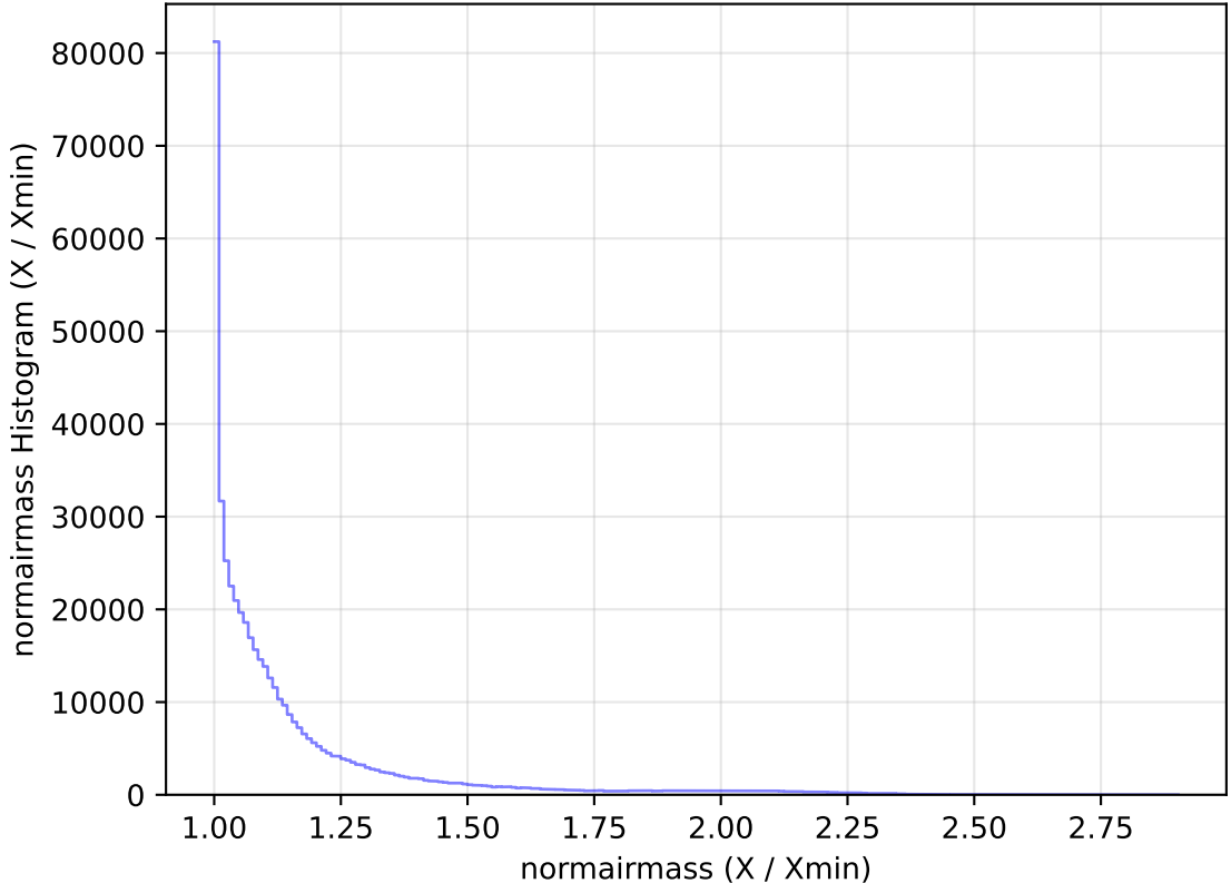
too_elab_heavy_r64_d3_griz_v3.4_10yrs All sky r band: normairmass Histogram
