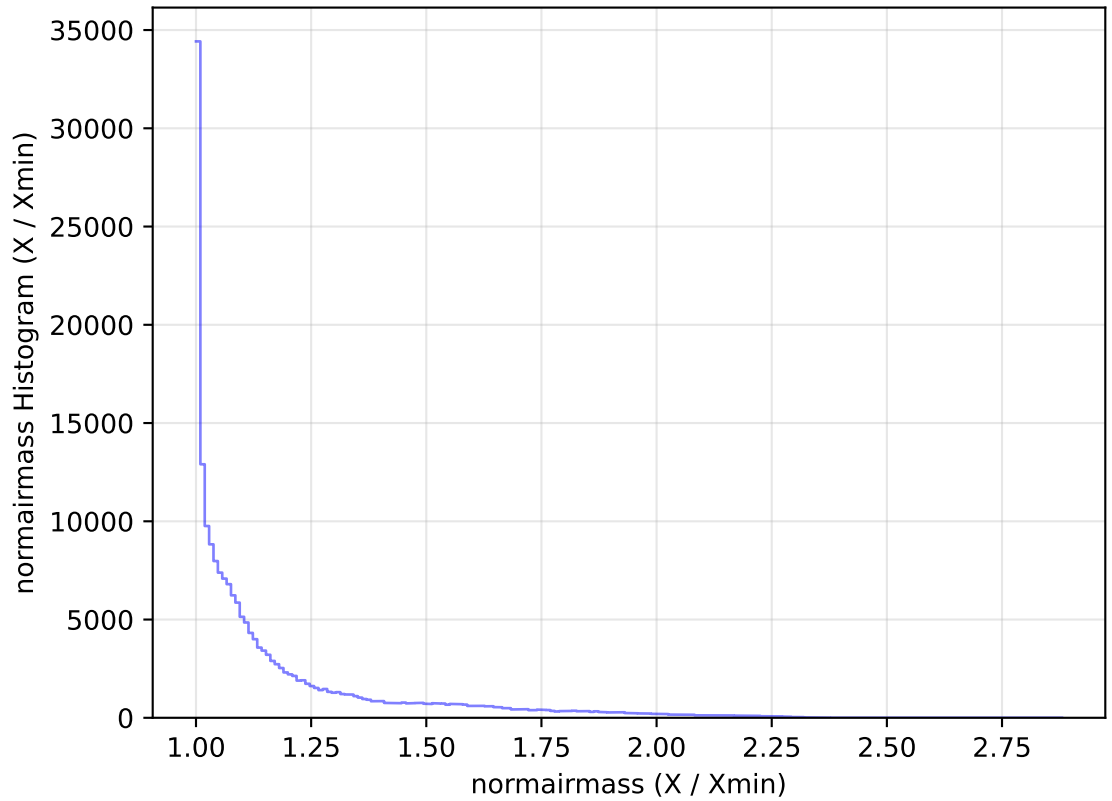
too_elab_heavy_r64_d3_griz_v3.4_10yrs All sky g band: normairmass Histogram
