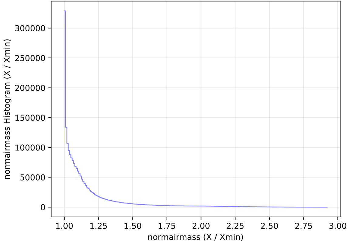
too_elab_heavy_r64_d3_griz_v3.4_10yrs All sky all bands: normairmass Histogram
