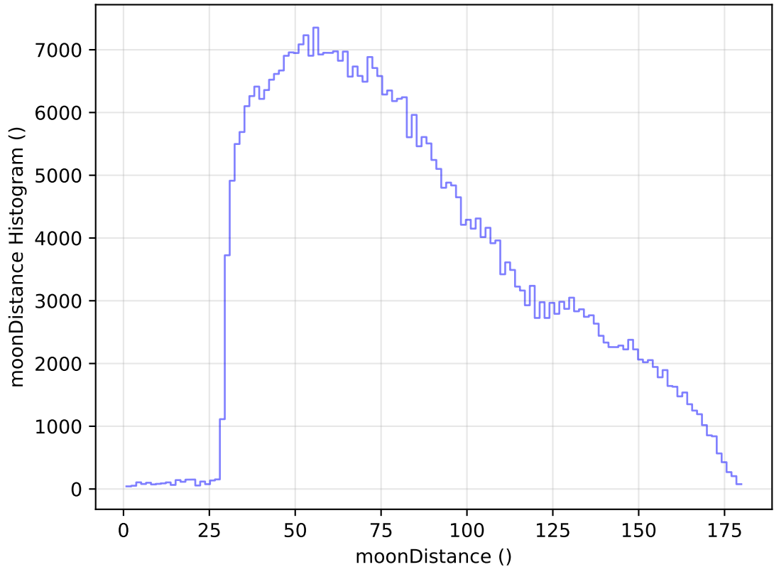
too_elab_heavy_r64_d3_griz_v3.4_10yrs WFD z band: moonDistance Histogram
