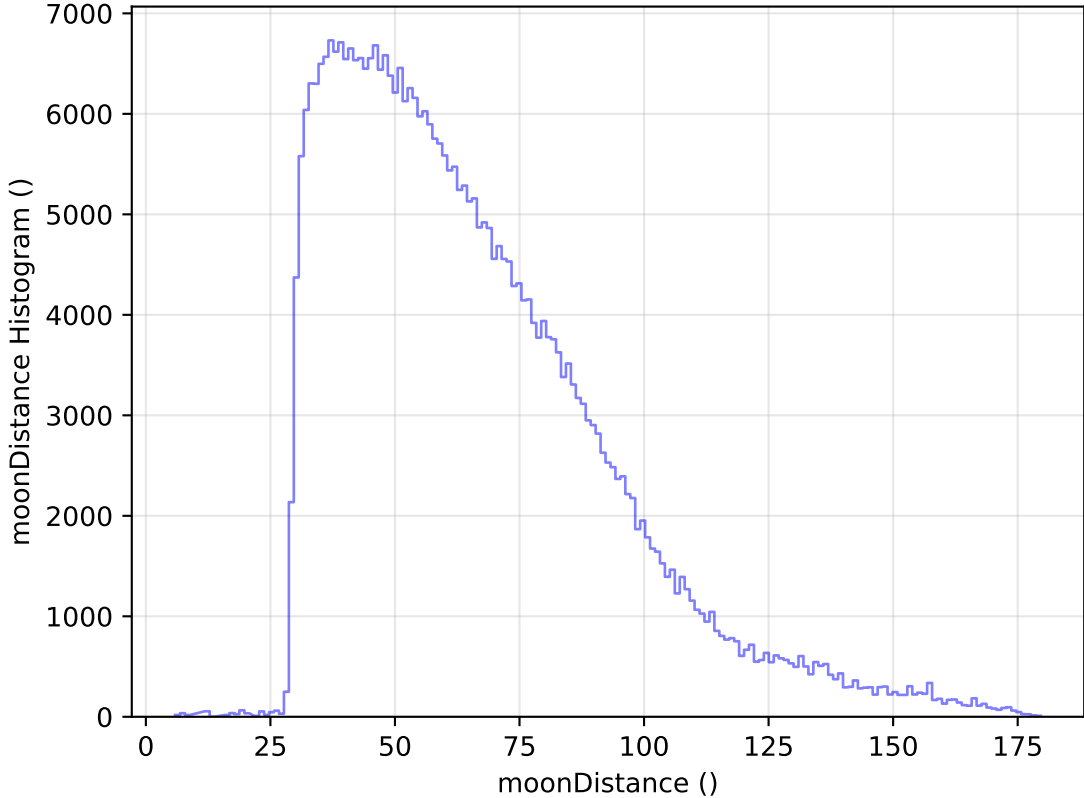
too_elab_heavy_r64_d3_griz_v3.4_10yrs WFD y band: moonDistance Histogram
