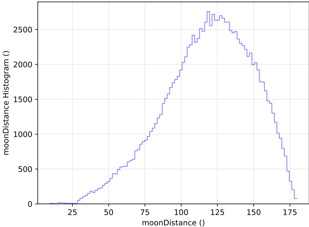
too_elab_heavy_r64_d3_griz_v3.4_10yrs WFD u band: moonDistance Histogram
