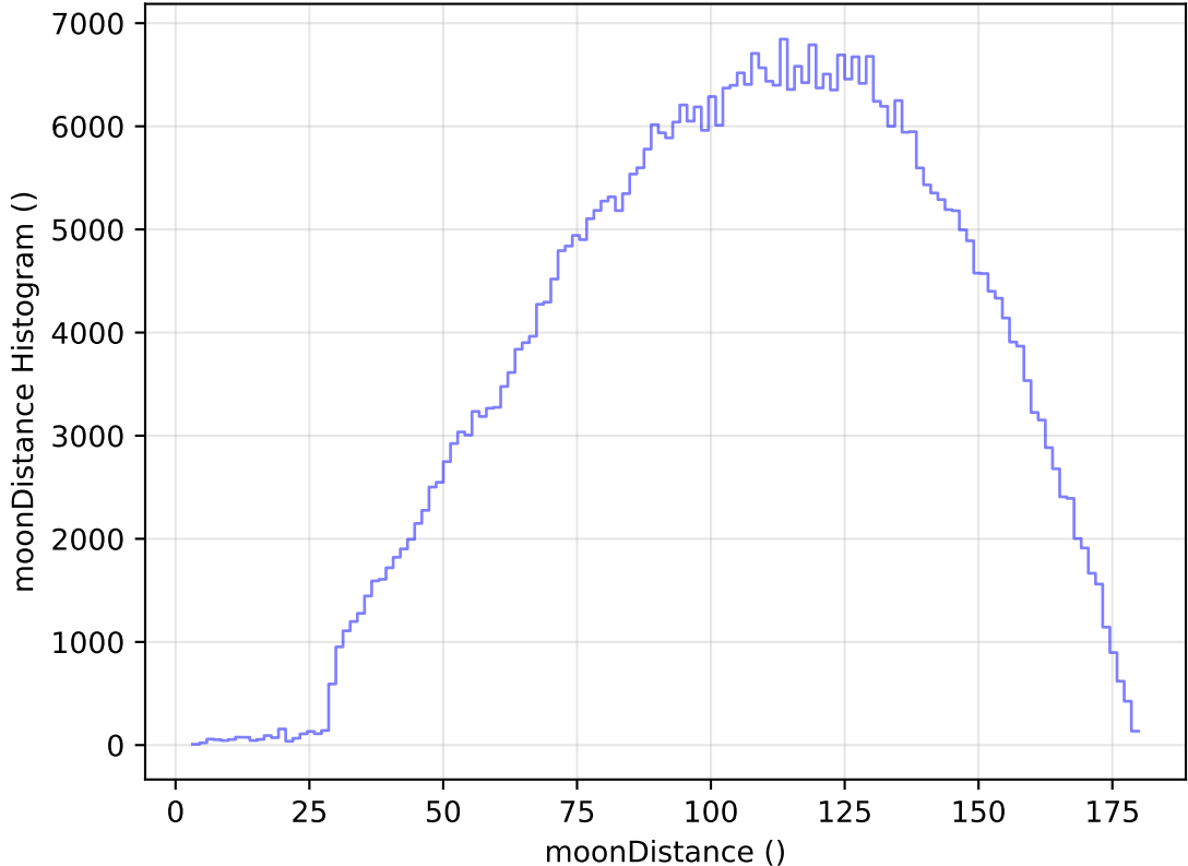
too_elab_heavy_r64_d3_griz_v3.4_10yrs WFD r band: moonDistance Histogram
