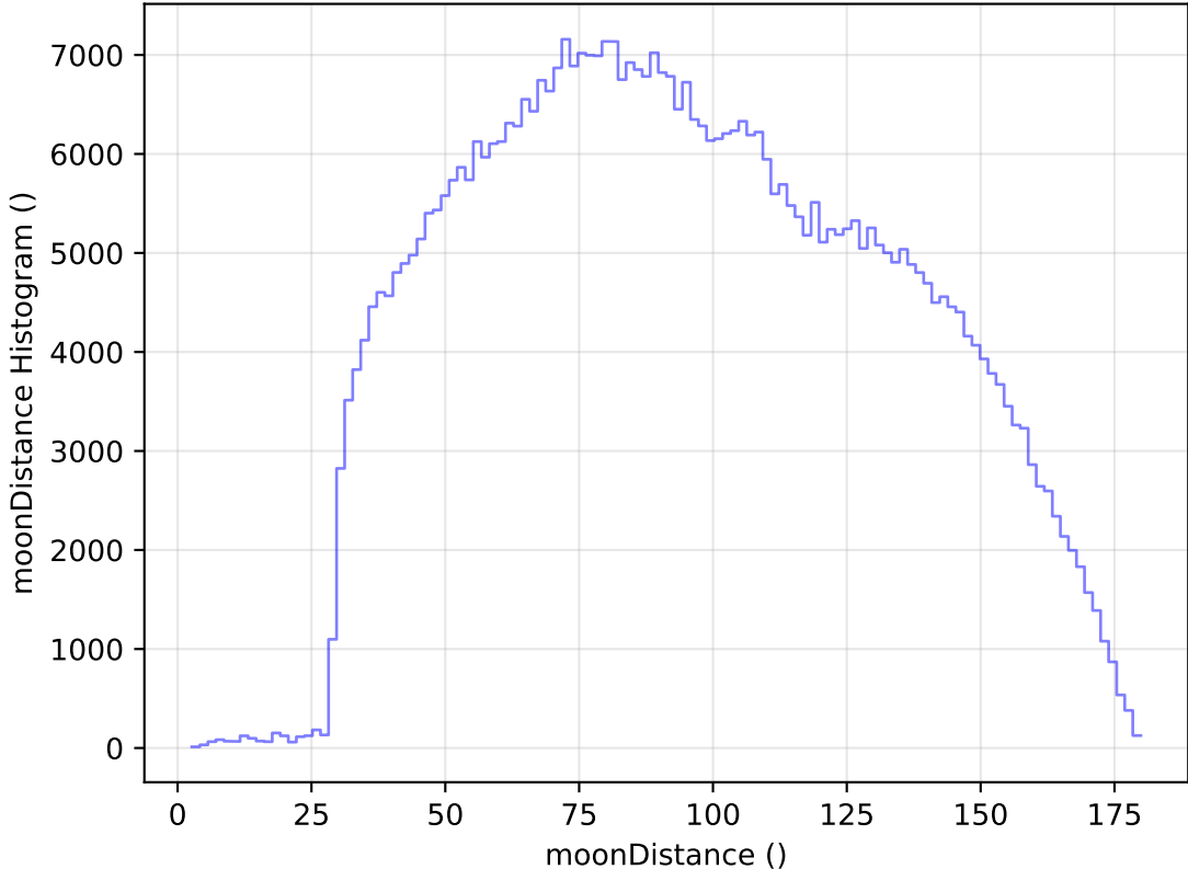
too_elab_heavy_r64_d3_griz_v3.4_10yrs WFD i band: moonDistance Histogram
