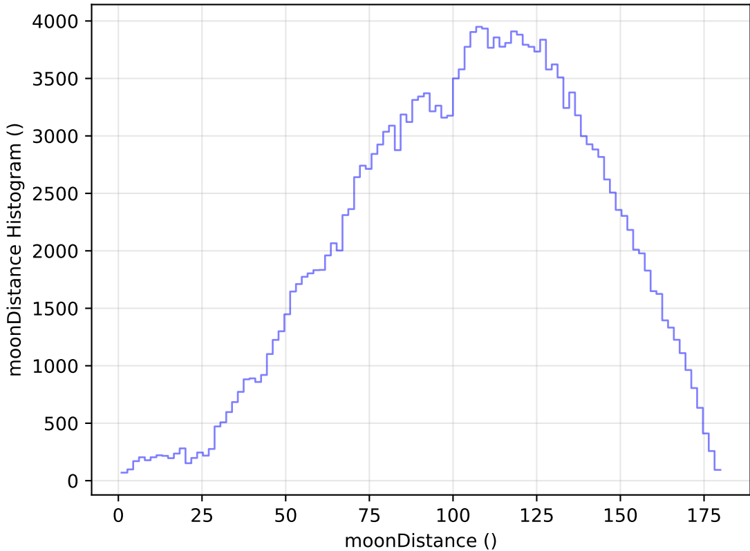
too_elab_heavy_r64_d3_griz_v3.4_10yrs WFD g band: moonDistance Histogram
