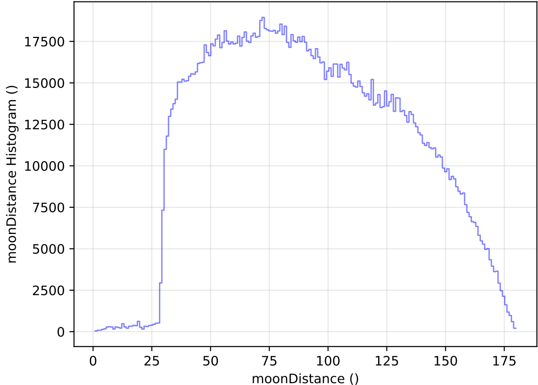
too_elab_heavy_r64_d3_griz_v3.4_10yrs WFD all bands: moonDistance Histogram
