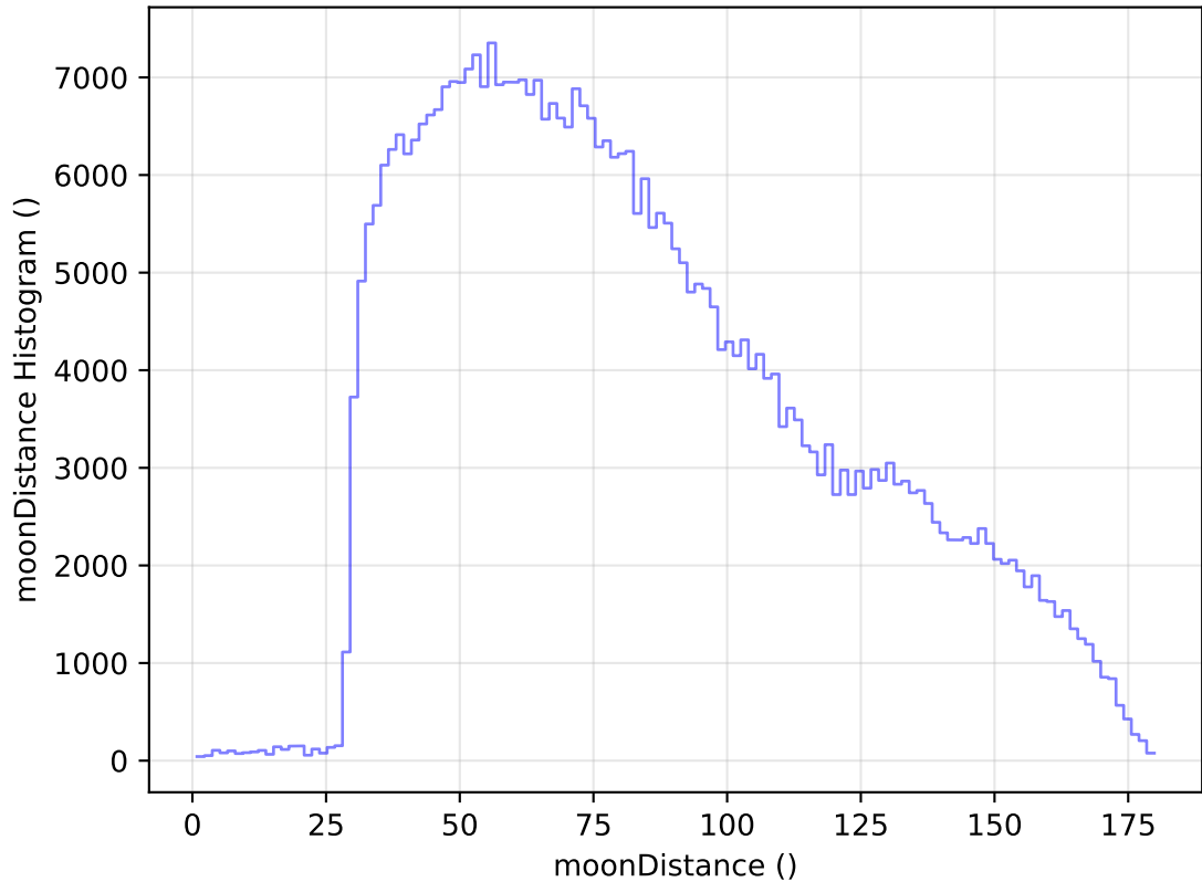
too_elab_heavy_r64_d3_griz_v3.4_10yrs All sky z band: moonDistance Histogram
