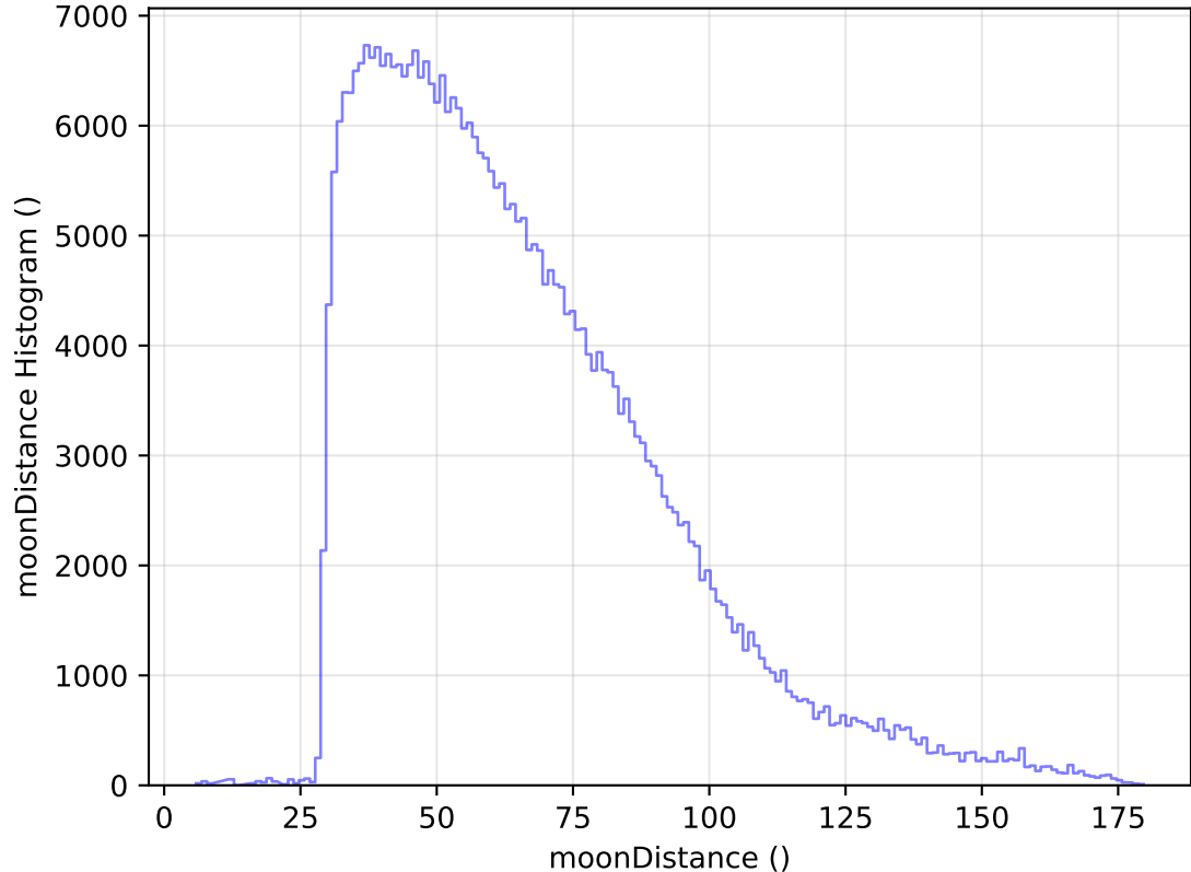
too_elab_heavy_r64_d3_griz_v3.4_10yrs All sky y band: moonDistance Histogram
