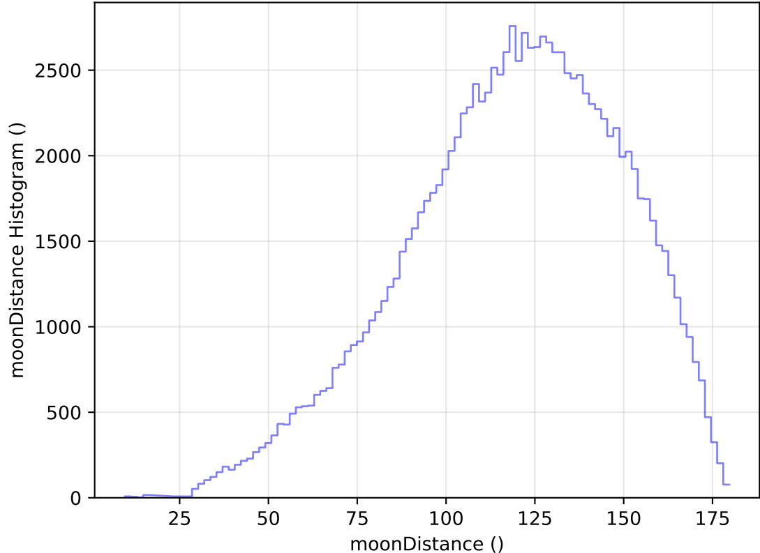
too_elab_heavy_r64_d3_griz_v3.4_10yrs All sky u band: moonDistance Histogram
