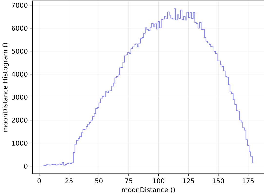
too_elab_heavy_r64_d3_griz_v3.4_10yrs All sky r band: moonDistance Histogram
