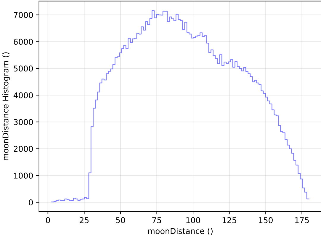
too_elab_heavy_r64_d3_griz_v3.4_10yrs All sky i band: moonDistance Histogram
