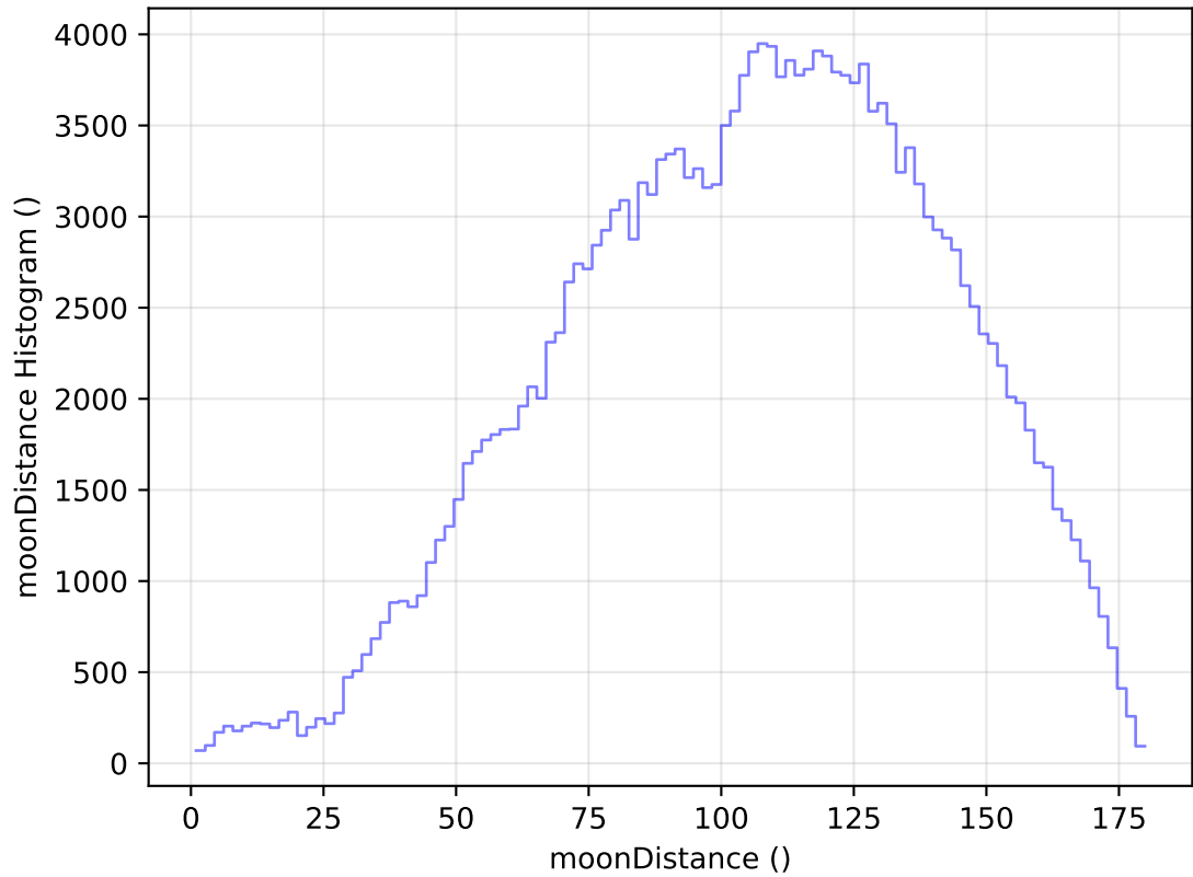
too_elab_heavy_r64_d3_griz_v3.4_10yrs All sky g band: moonDistance Histogram
