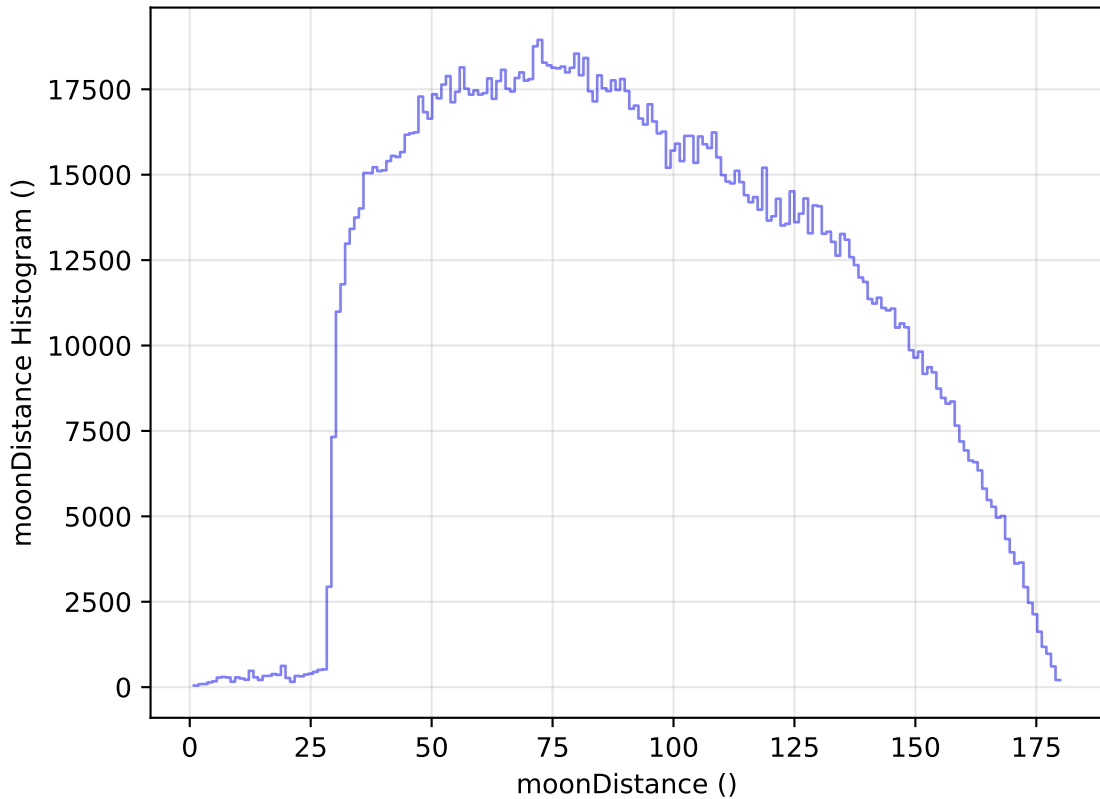
too_elab_heavy_r64_d3_griz_v3.4_10yrs All sky all bands: moonDistance Histogram
