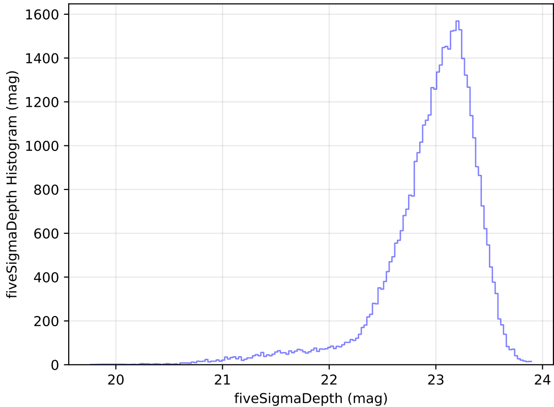
too_elab_heavy_r64_d3_griz_v3.4_10yrs Yr 1 z band: fiveSigmaDepth Histogram
