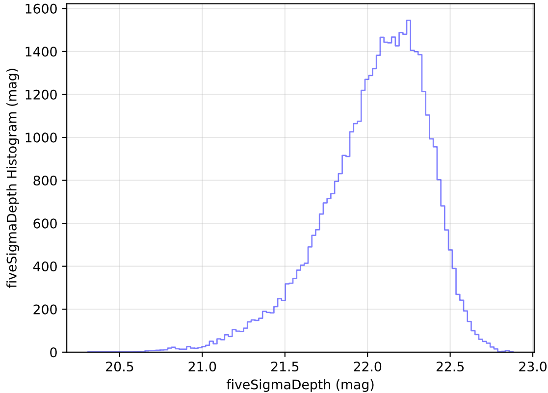
too_elab_heavy_r64_d3_griz_v3.4_10yrs Yr 1 y band: fiveSigmaDepth Histogram
