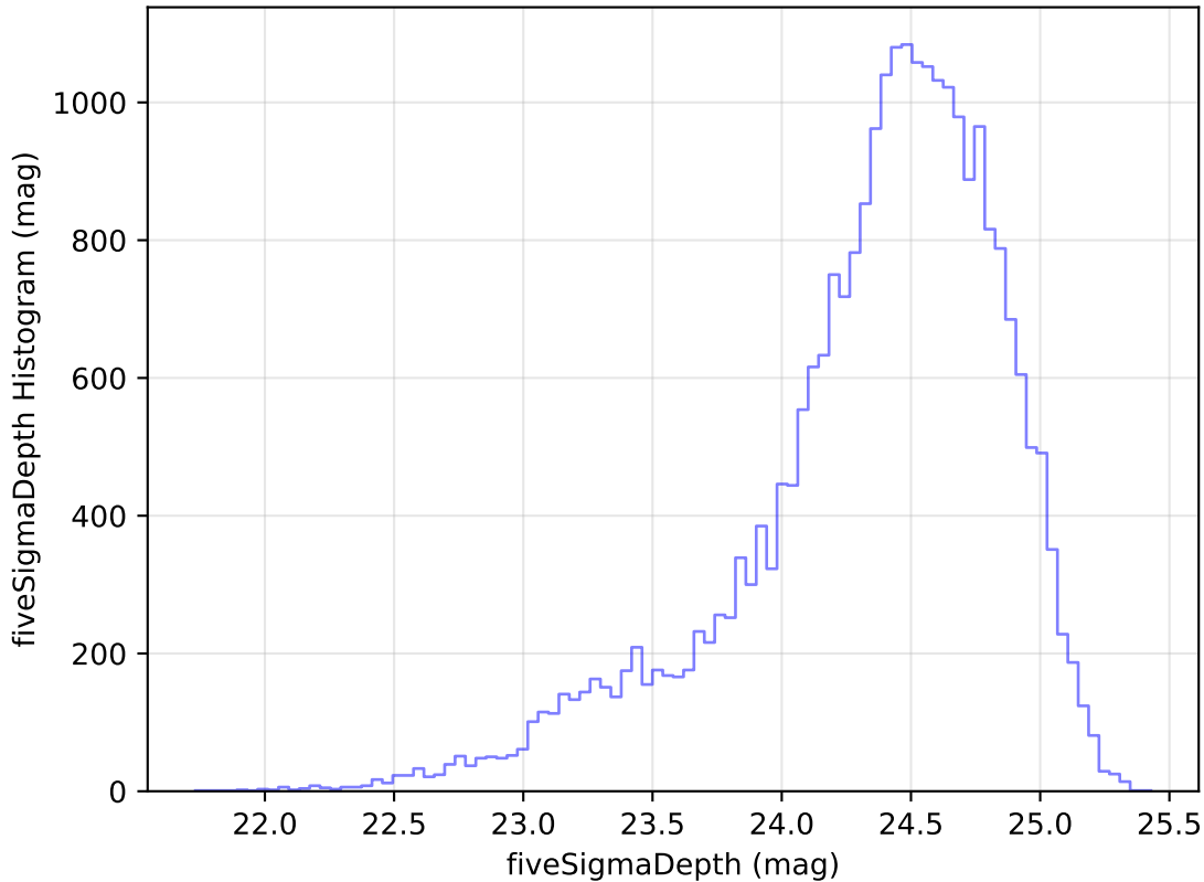
too_elab_heavy_r64_d3_griz_v3.4_10yrs Yr 1 g band: fiveSigmaDepth Histogram
