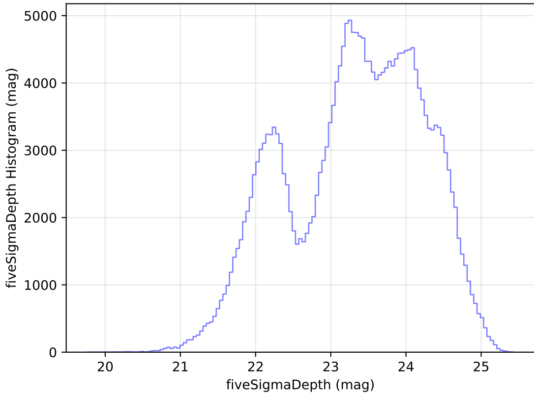
too_elab_heavy_r64_d3_griz_v3.4_10yrs Yr 1 all bands: fiveSigmaDepth Histogram
